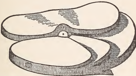
FIG. 7.—THE GALACTIC FLAT RING MODIFIED IN ACCORDANCE WITH THE OBSERVED PECULIARITIES OF THE MILKY WAY.
